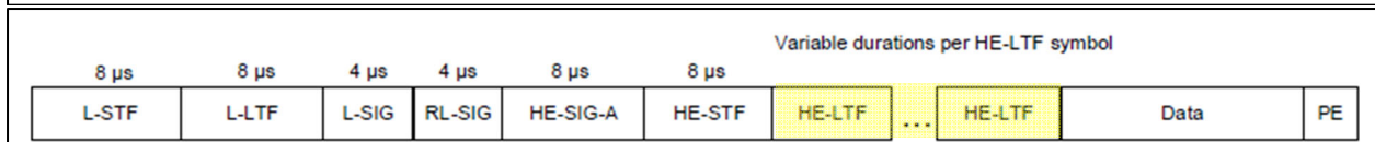
Figure 27-11—HE TB PPDU format
